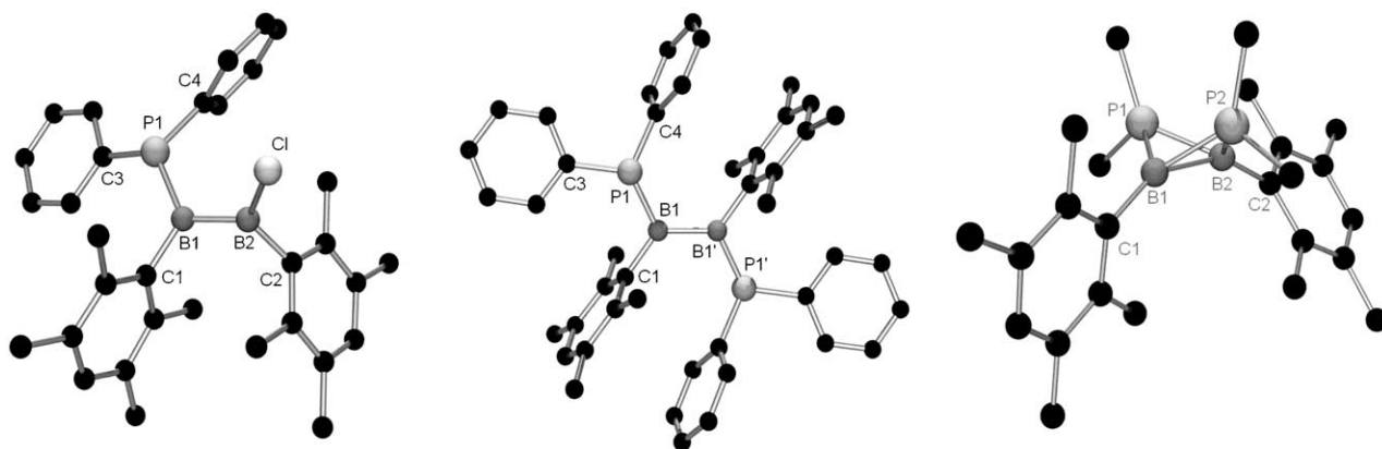
Figure 1. Molecular structure of 7 BP c in the solid state (left; hydrogen atoms are omitted for clarity). Selected bond lengths [Å] and angles [°]: P1–B1 1.845(2), B1–B2 1.687(3); B1–P1–C4 115.78(9), B1–P1–C3 119.83(10), C4–P1–C3 107.48(9), P1–B1–B2 119.85(15), P1–B1–C1 121.21(14), B2–B1–C1 118.65(16), B1–B2–C1 119.86(15), B1–B2–C2 121.57(17), Cl–B2–C2 118.50(15). Molecular structure of 1 BP c in the solid state (center; hydrogen atoms are omitted for clarity). Selected bond lengths [Å] and angles [°]: P1–B1 1.8346(16), B1–B1' 1.712 (3); B1–P1–C4 121.73(6), B1–P1–C3 121.69(7), C4–P1–C3 107.15(7), P1–B1–B1' 117.03(12), P1–B1–C1 116.08(9), B1'–B1–C1 126.44(15). Molecular structure of 3 BP c in the solid state (right; hydrogen atoms and noncoordinated atoms of the phenyl groups on the phosphorus atoms are omitted for clarity). Selected bond lengths [Å]: B1–B2 1.971(2), B1–P1 1.8874(15), B1–P2 1.8858(15), B2–P1 1.8819(16), B2–P2 1.8870(16).
